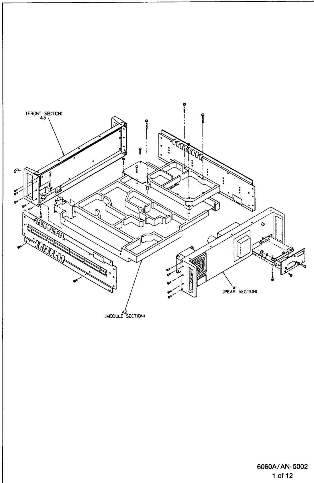
Figure 5-1. 6060A/AN Final Assembly (cont)
